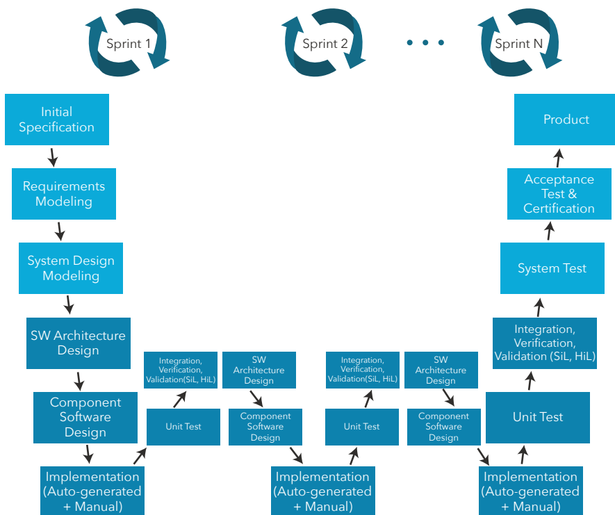
Figure 3: W-Model for Agile Workflow
