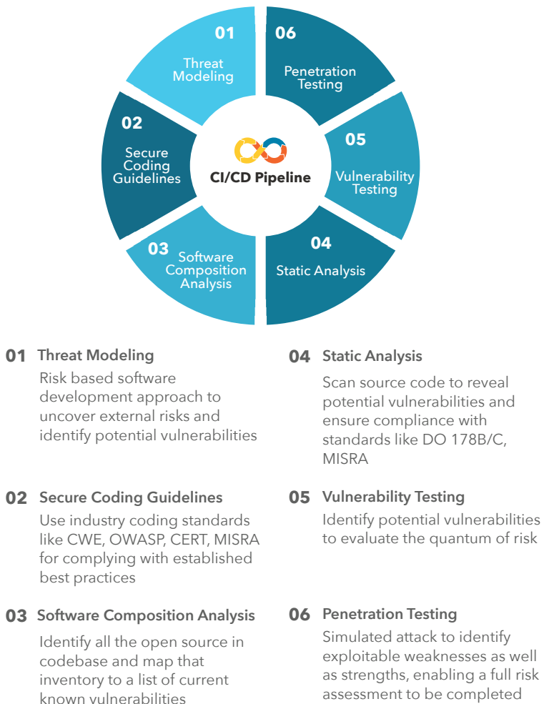
Figure 4: Automated Security Checks in CI/CD Pipeline
