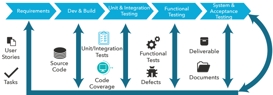
Figure 5: Bi-directional Requirement Traceability
