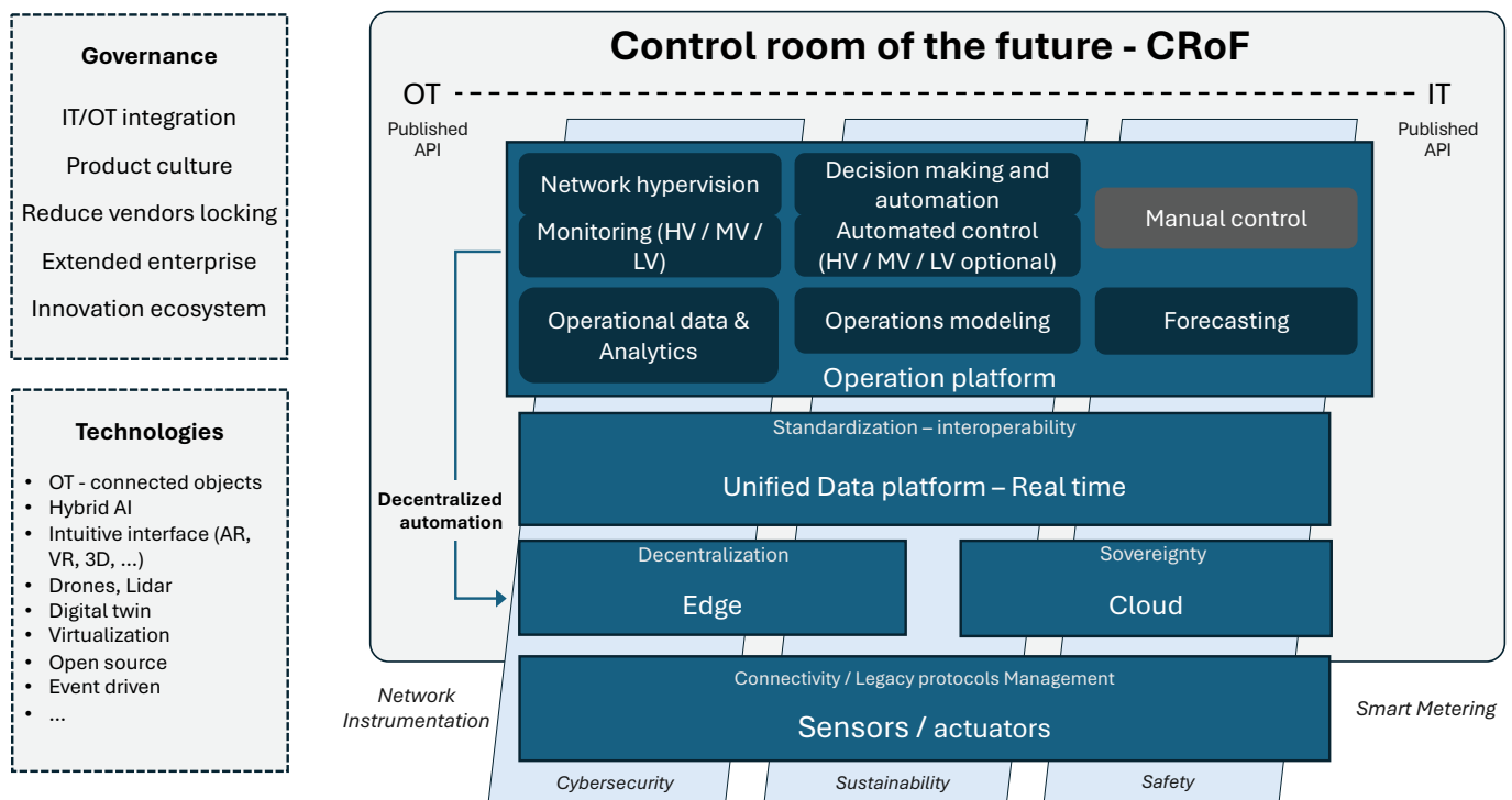
Figure 3: Typical Architecture level 1
